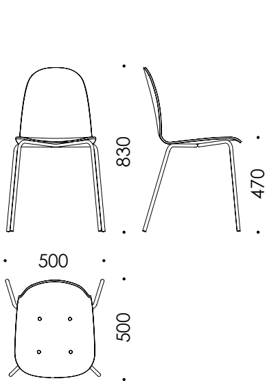
NamNam Contract (stackable) Painted, natural or stained wood Front upholster possible Painted metal frame Painted or brass fix screws Optional linking bracket.
